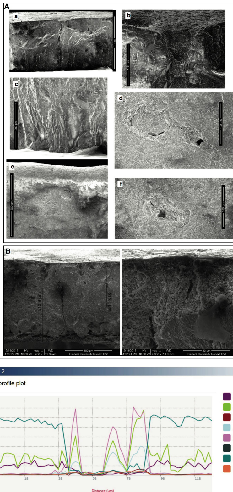
Extended Data Figure 9 | Analysis of putative Genyornis oological eggshell material. A , Scanning electron micrographs of sample 1 from square 4C, quadrat B, spit 18. Aa , view of a fresh broken edge showing a smooth eroded-out surface (upper), a section through a pore canal; Ab , detail of the pore canal opening showing the material filling pore; Ac , detail of the inner layer 1 and smooth inner surface of the shell showing that it is slightly eroded, so that the tips of the mammillary cones of layer 1 are lost; Ad , outer surface of the shell showing an elongated pair of pore canal openings occluded by material; Ae , outer surface of the shell showing the rounded eroded edge of the fragment; Af , outer surface of the shell and another opening to a pore canal showing its elongated nature
